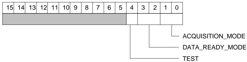
Fig. 3.16: Control Register 2
