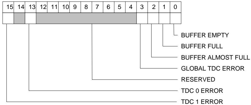
Fig. 3.15: Status Register 2
