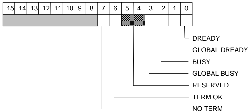
Fig. 3.9: Status Register 1
