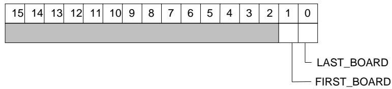
Fig. 3.14: Control Register 1
