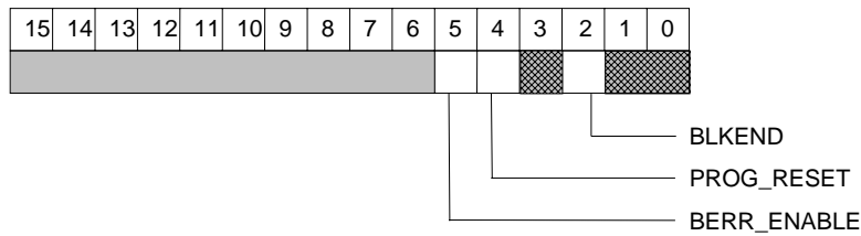
Fig. 3.10: Control Register 1
